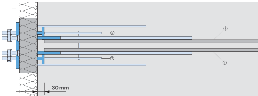
Plan view – On-site cast concrete
