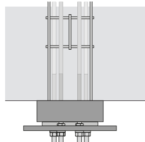
f correct: elements aligned on one axis
