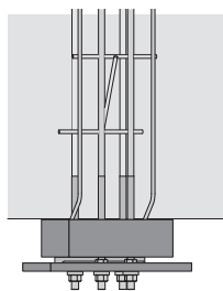
e incorrect: displacement; horizontally to the concrete edge – forwards or backwards
